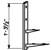
DETAIL 'A' TYPICAL CABLE RACK AND SUPPORTS
